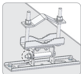
Fig 1. Mounting Down Bracket
