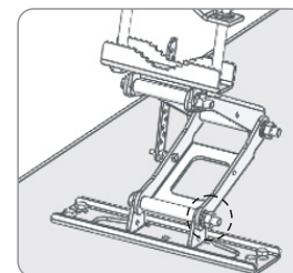
Fig 3. Mounting Upper Bracket
