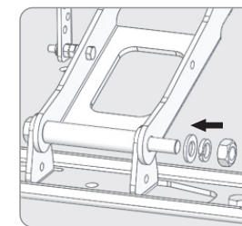
Fig 4. Detail Mounting
