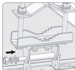
Fig 2. Detail Mounting
