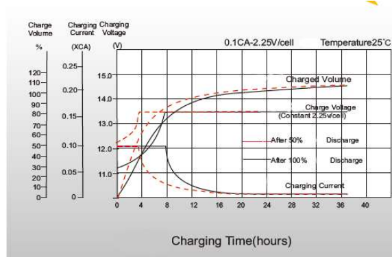
Float charging characteristic(25°C)
