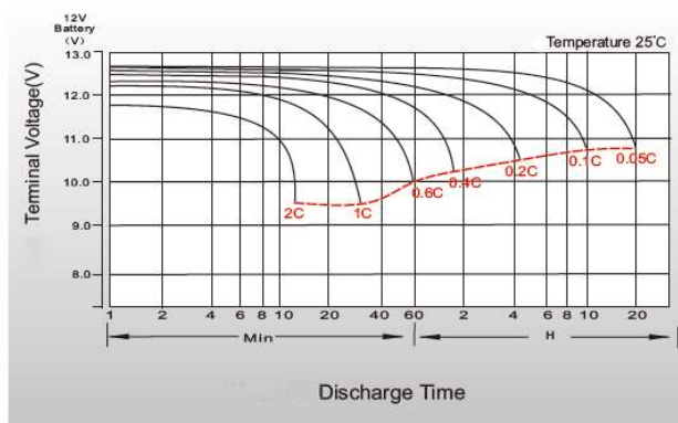
Discharge characteristic(25°C)
